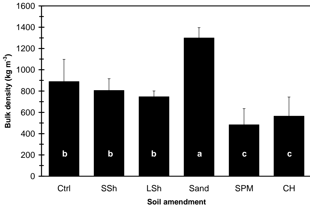
Figure 2. Effects of small diameter expanded shale (SSh), large diameter expanded shale (LSh), sand, sphagnum peat moss (SPM), and cottonseed hulls (CH) on bulk density of Austin silty clay (Ctrl) soil seven months after application ( 1000 \text{ kg m}^{-3} = 62 \text{ lb ft}^{-3} ). Columns with the same letter are not statistically different at the 0.05 level of probability, n=6 .
